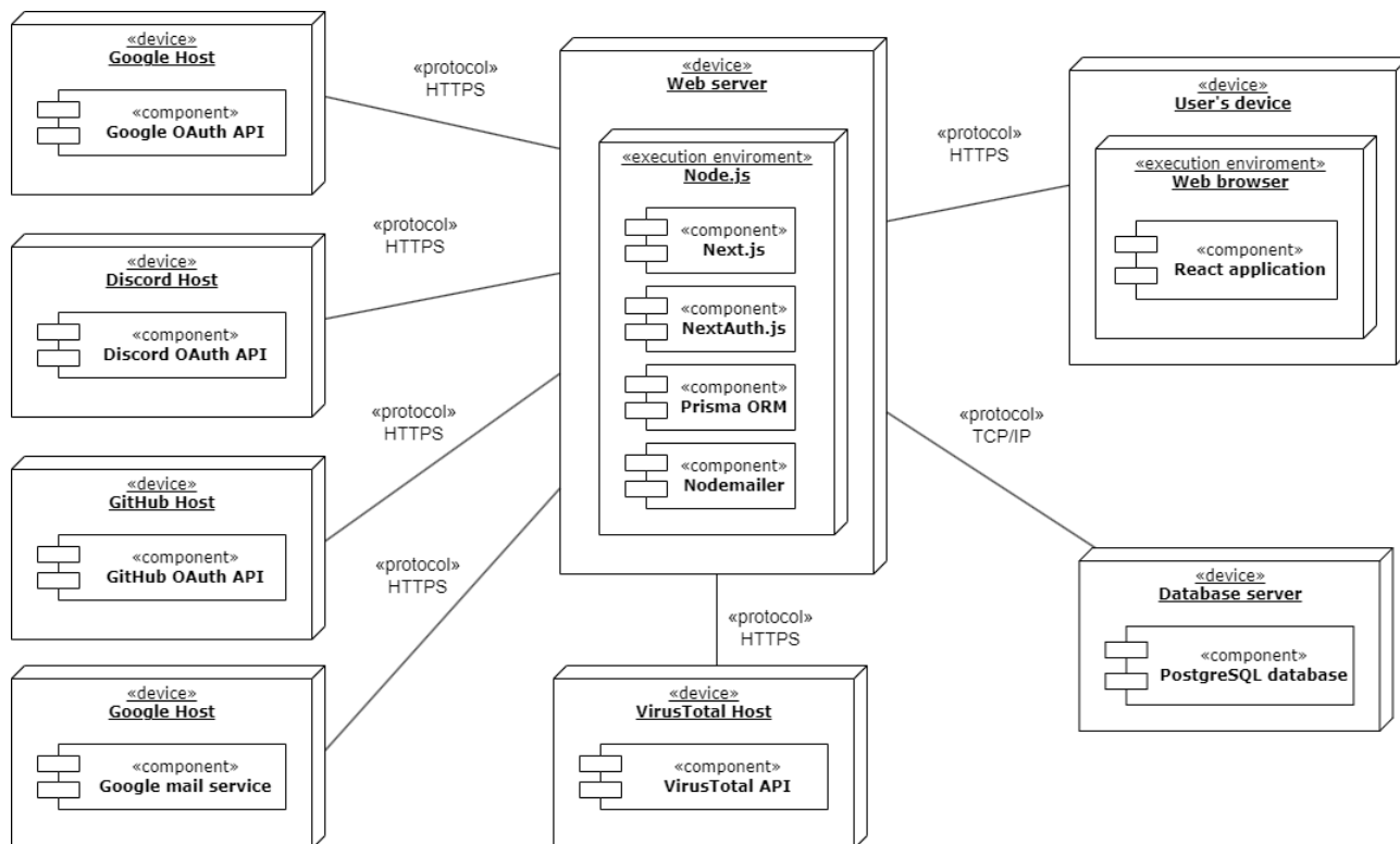
Figure 2 – Software deployment diagram
